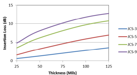
JCS-X Insertion Loss @3GHz
